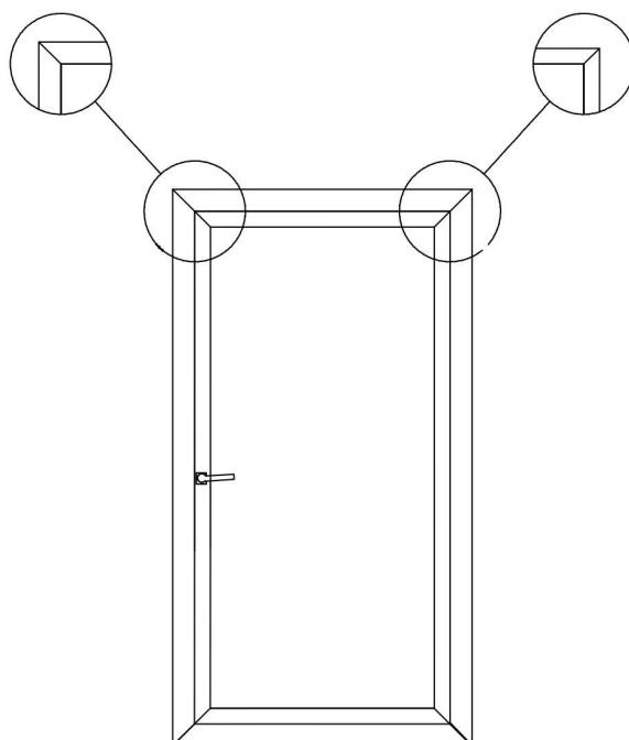
45° OUTER FRAME
