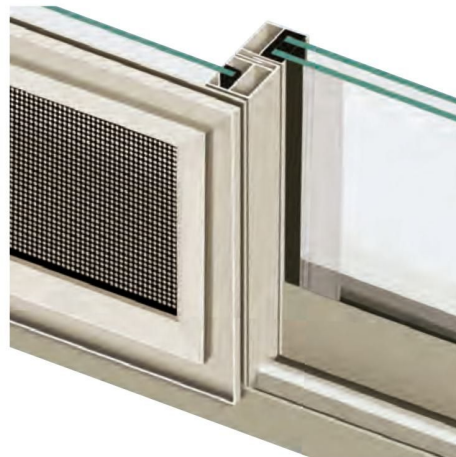
LUXURY SERIES L2½
