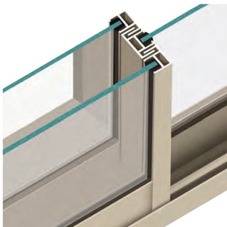
SLIM SERIES SW3
