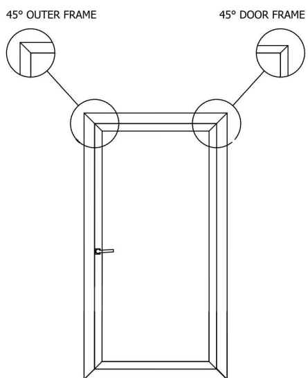
SINGLE CASEMENT DOOR
